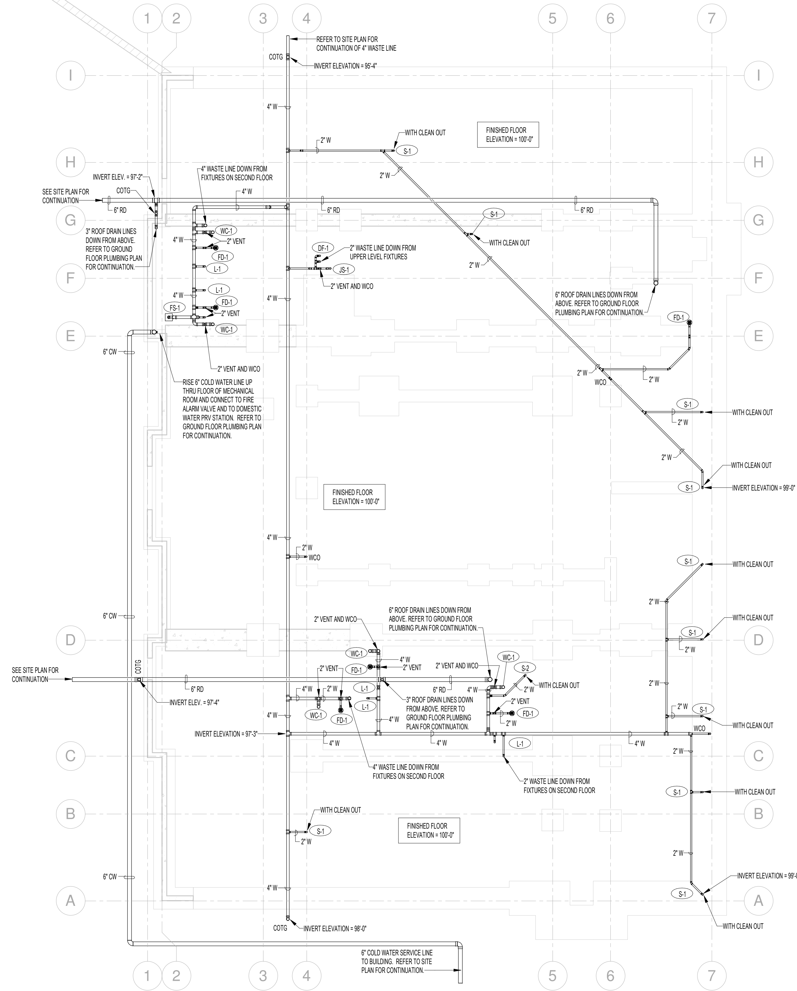
FOUNDATION PLUMBING PLAN SCALE: 1/8" = 1'-0"
