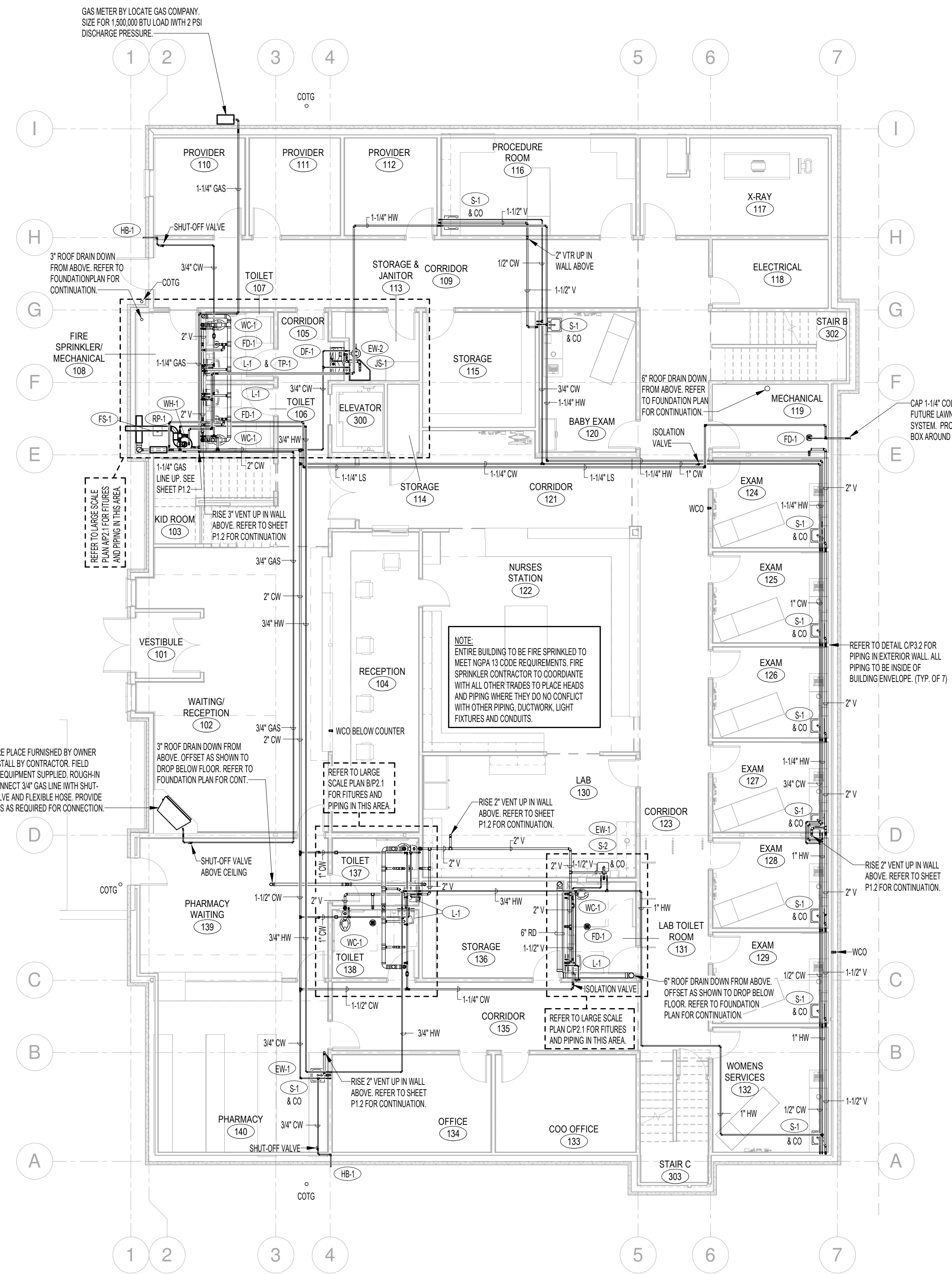
GROUND FLOOR PLUMBING PLAN SCALE: 1/8" = 1'-0"
